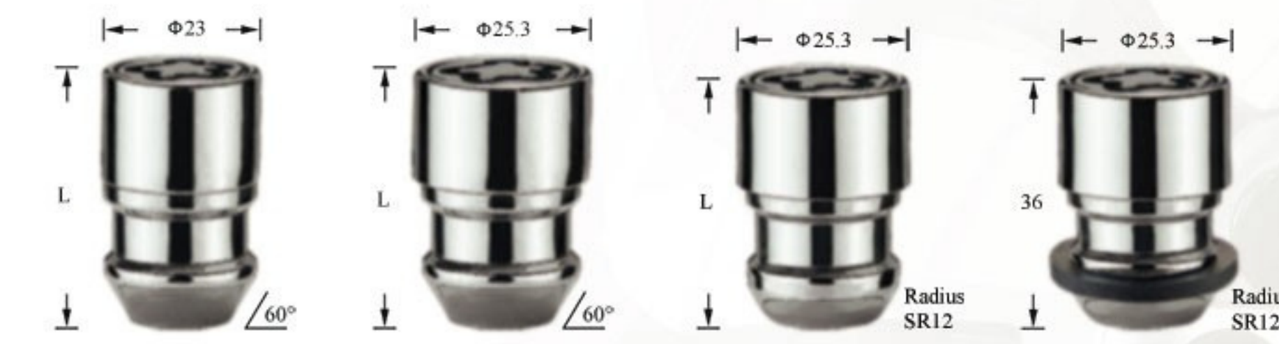
46800 (L=30) 46304 (L=28) 46306 (L=30) 46500 (L=36) 46622 46801 (L=33) 46307 (L=33) 46300 (L=36) 46501 (L=38) 46301 (L=38) 46302 (L=42) 46303 (L=51) 46305 (L=58)
